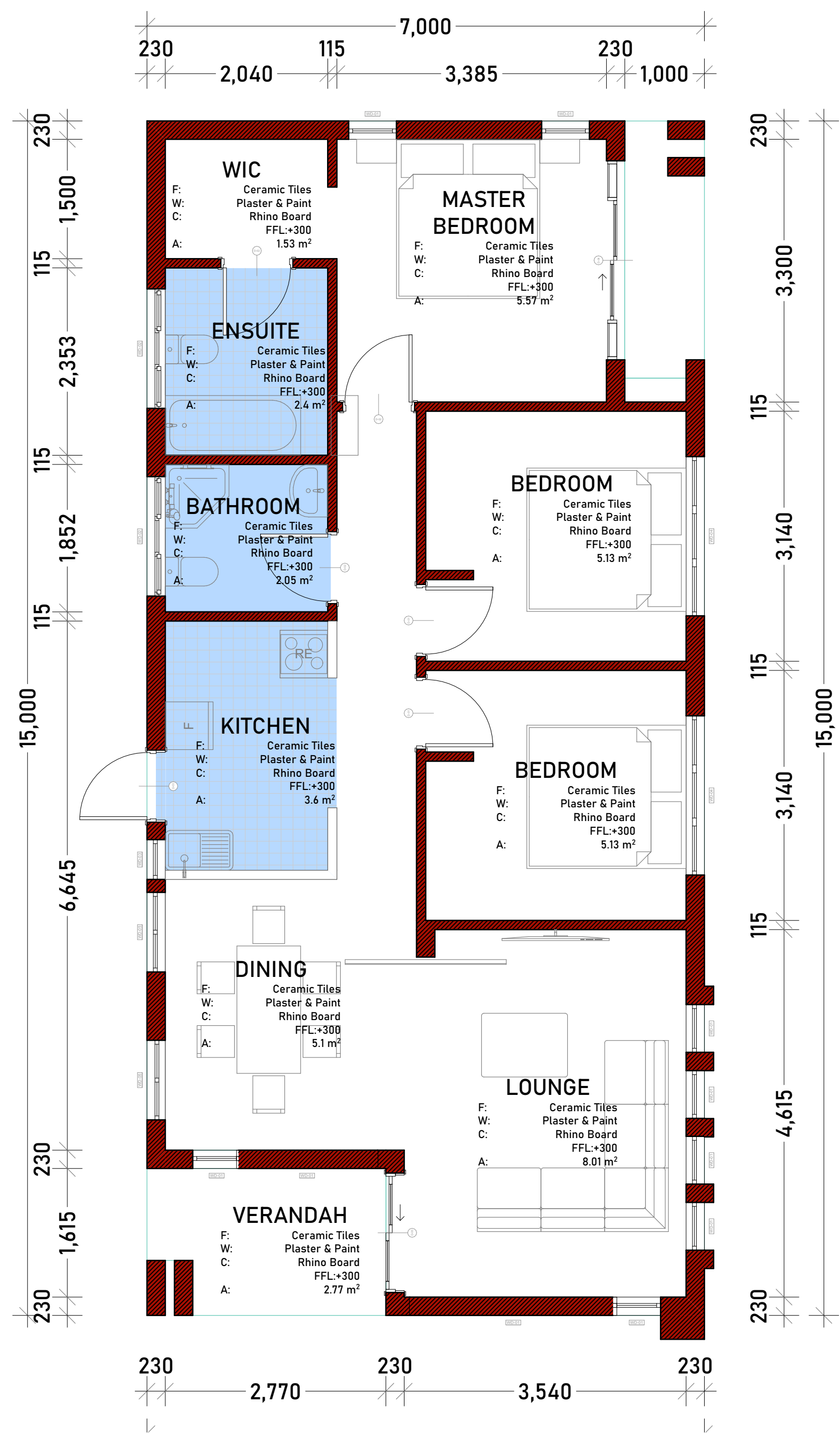
0. UNIT 05 FLOOR PLAN 1:50
